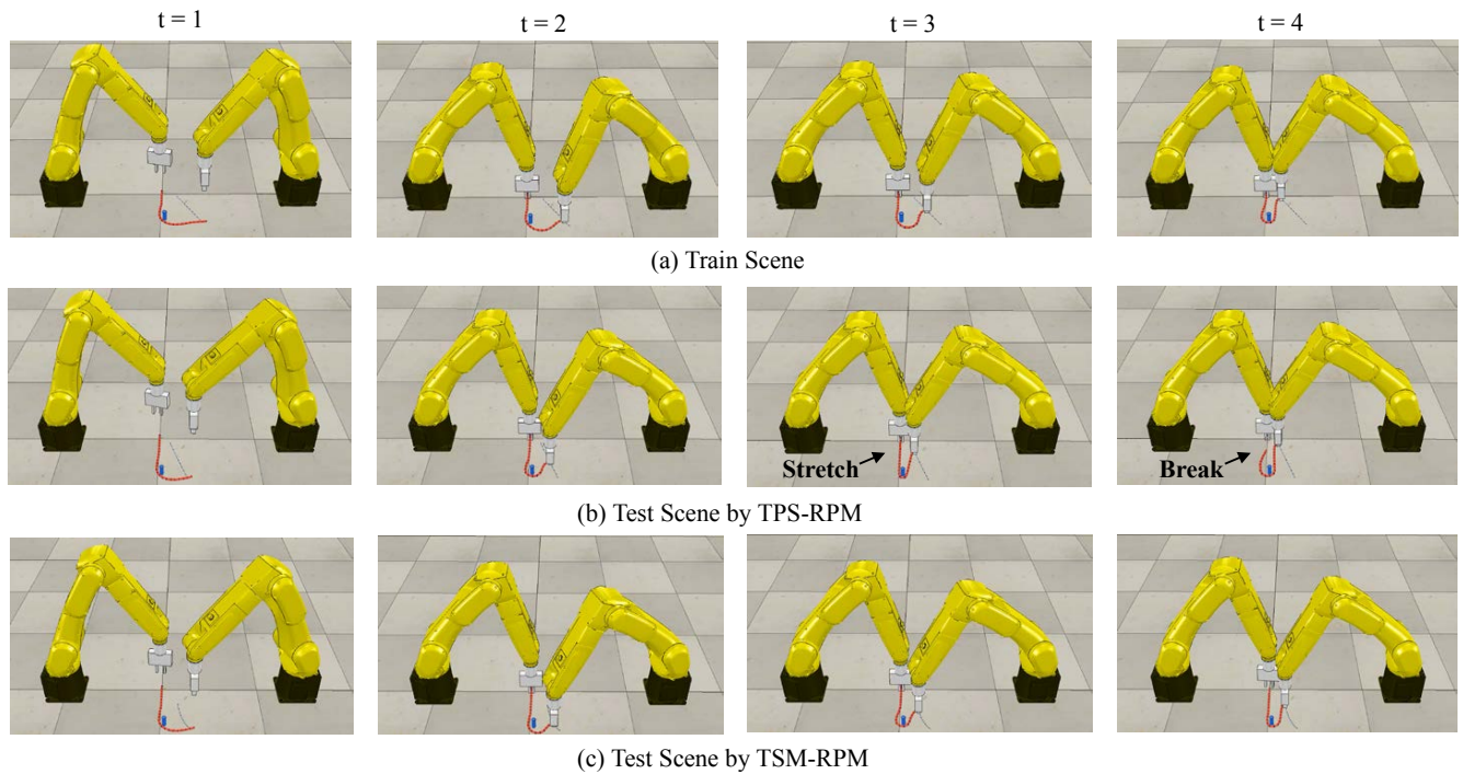
Fig. 7. Bending the rope ninety degrees around the shaft. The initial shape of the rope is changed at test. TPS-RPM overstretches the test rope at time frame t = 3 and the rope severs at t = 4 . In contrast, TSM-RPM succeeds and does as well as training without incurring overstretching.
